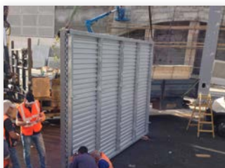
Self-carrying back structure for gantry installation
