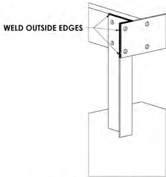
LEFT FRONT OF BACKING PLATE
