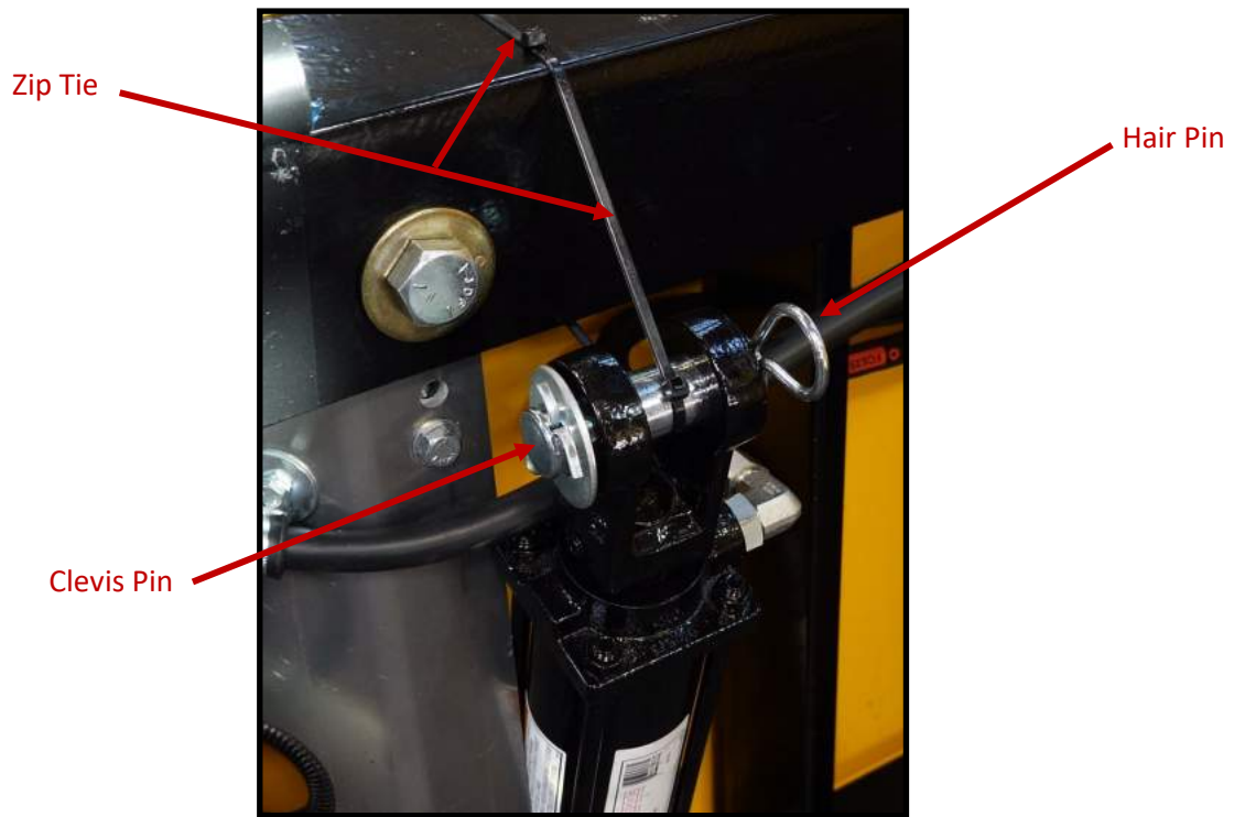
Hydraulic Cylinder
