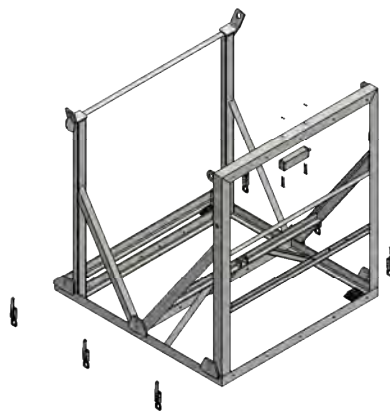
Locking Latches (6)
